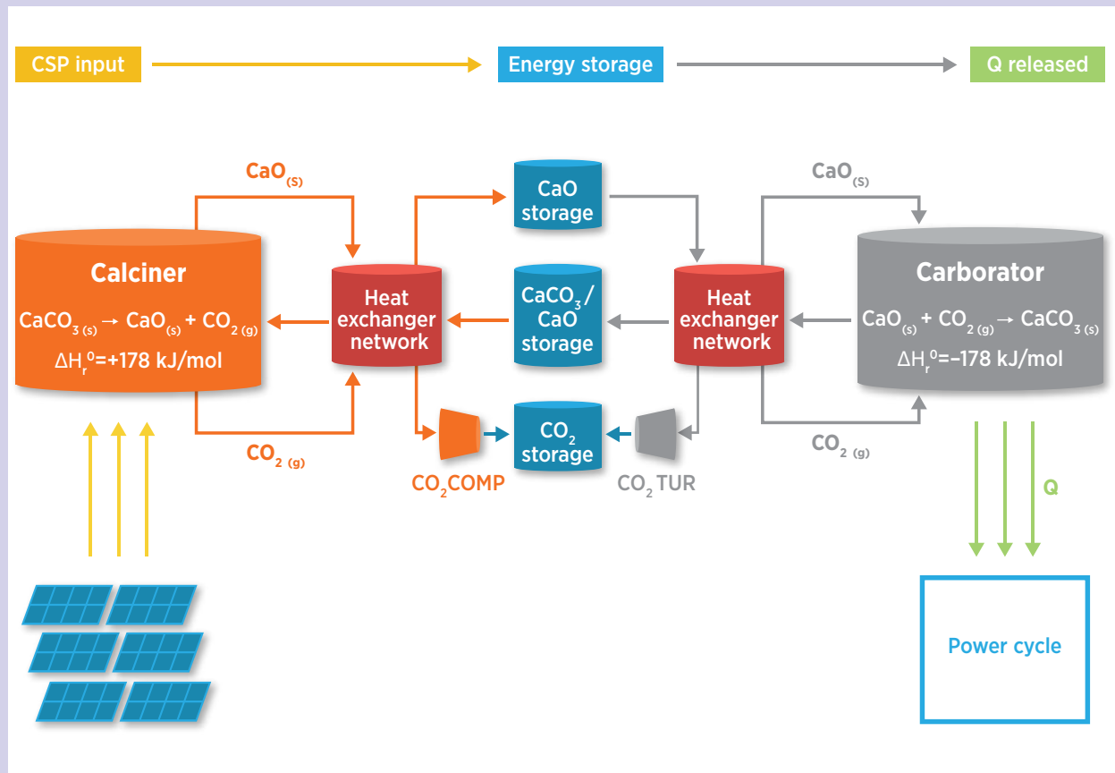
Figure 50. CSP-CaL integration for thermochemical energy storage
