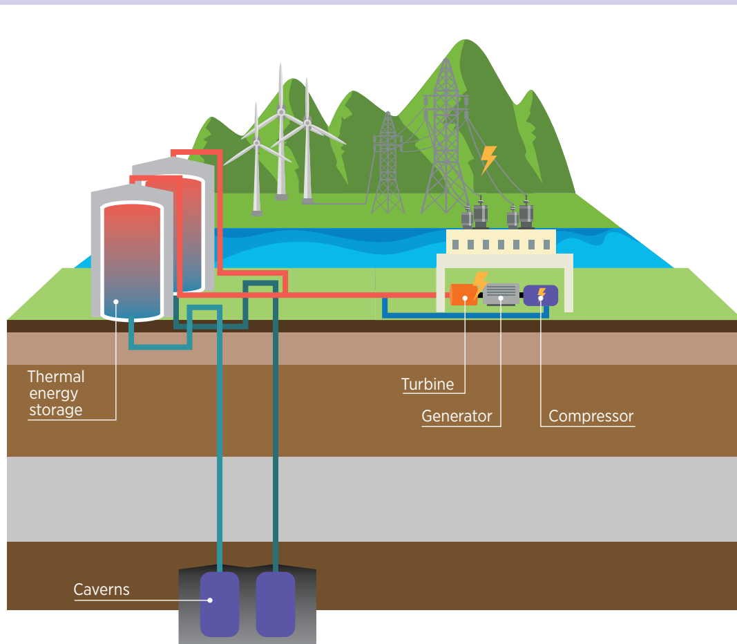
Figure 34: Diagram of a proposed A-CAES site
