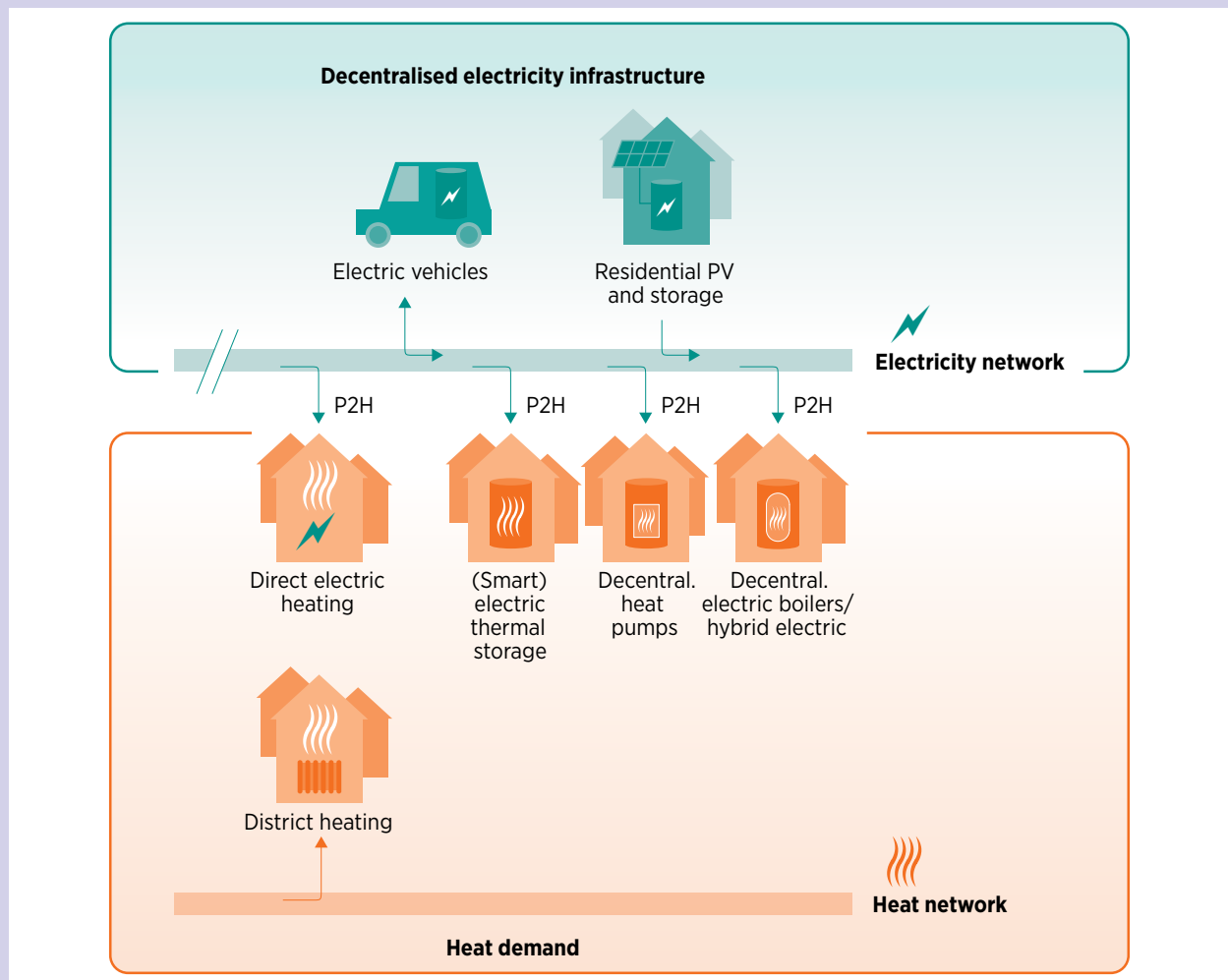
Figure 22. Overview of an integrated and decentralised electricity infrastructure to meet power and heat demand flexibly
