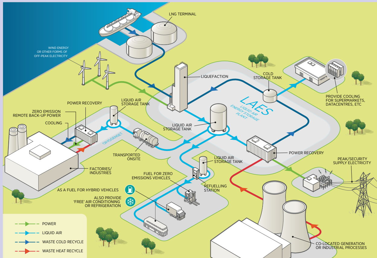
Figure 44. A vision for the use of LAES in the integrated cold chain of the future
