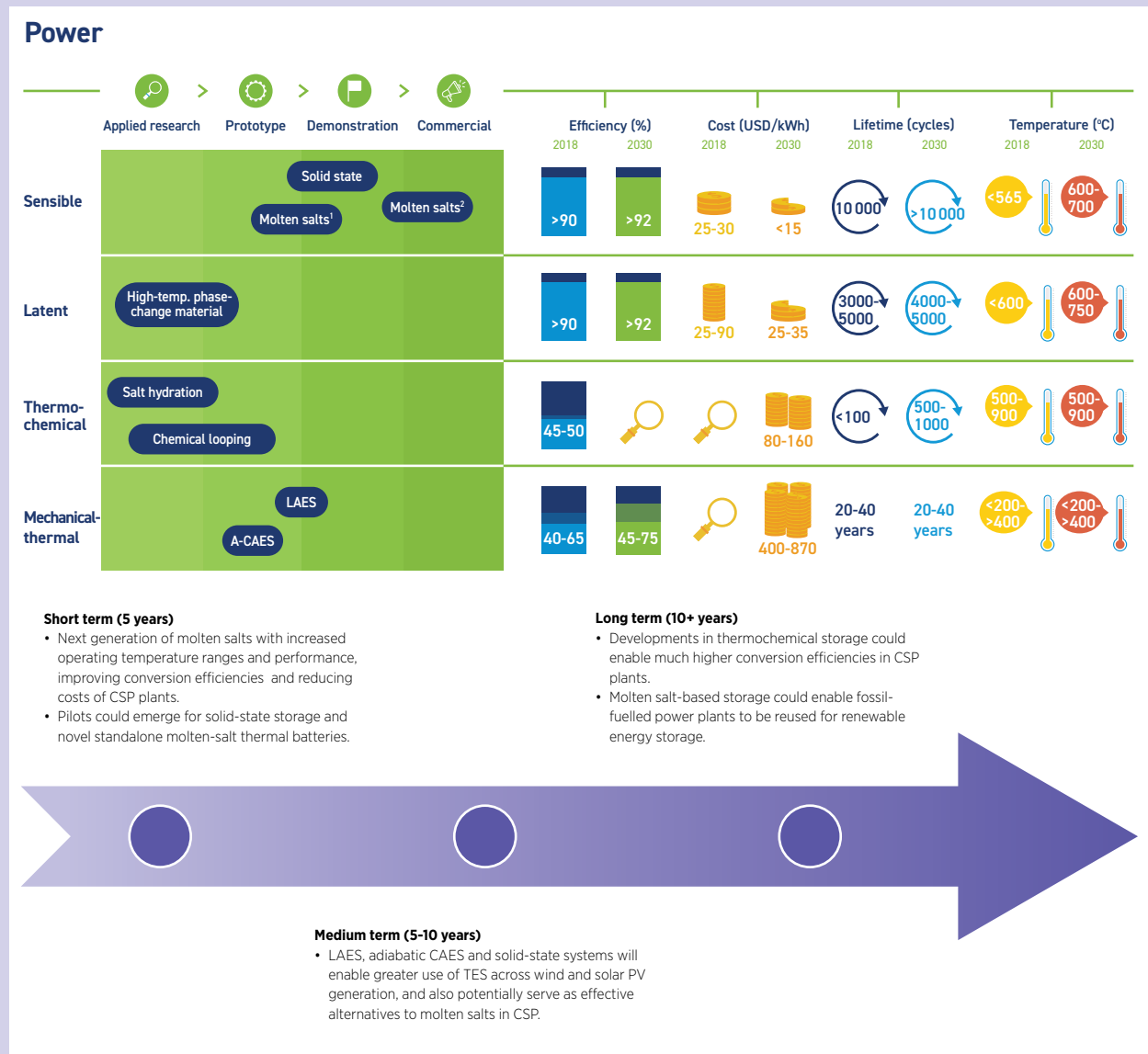
Figure 7: TES technology status and innovation outlook in the power sector
