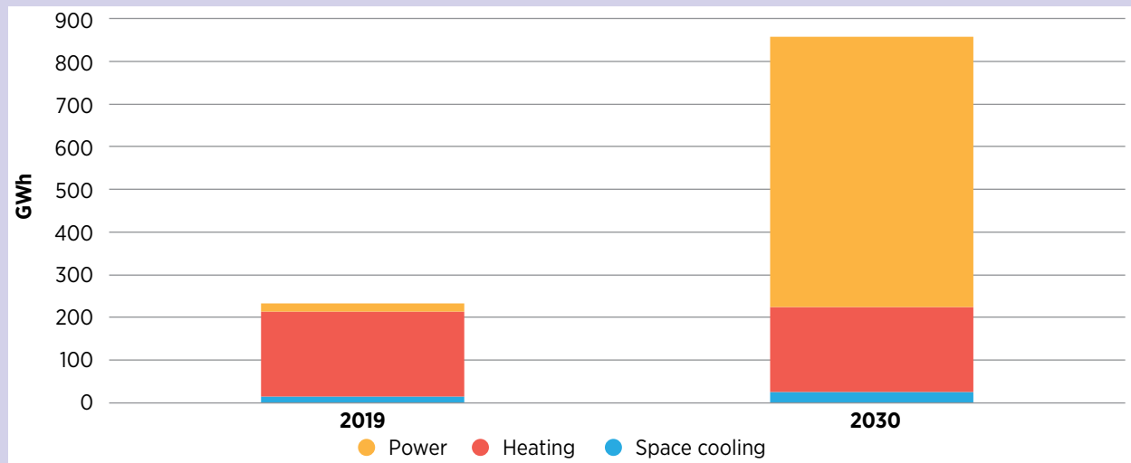
Figure 21: Installed TES capacity projections
