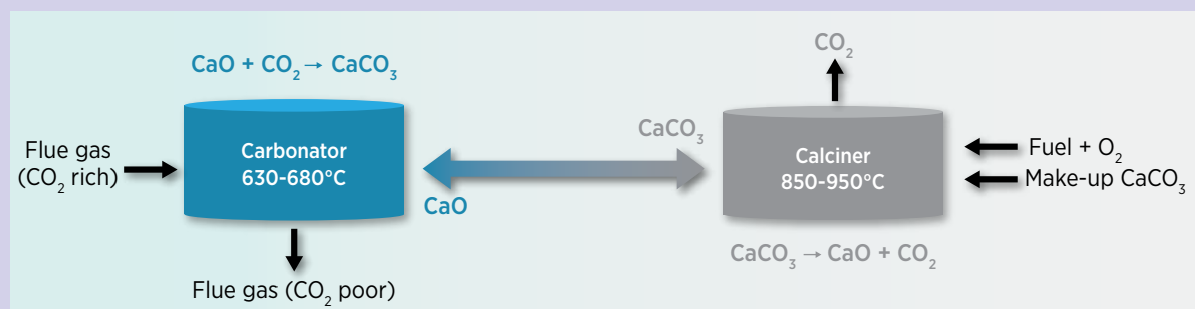
Figure 31: CaL process scheme
