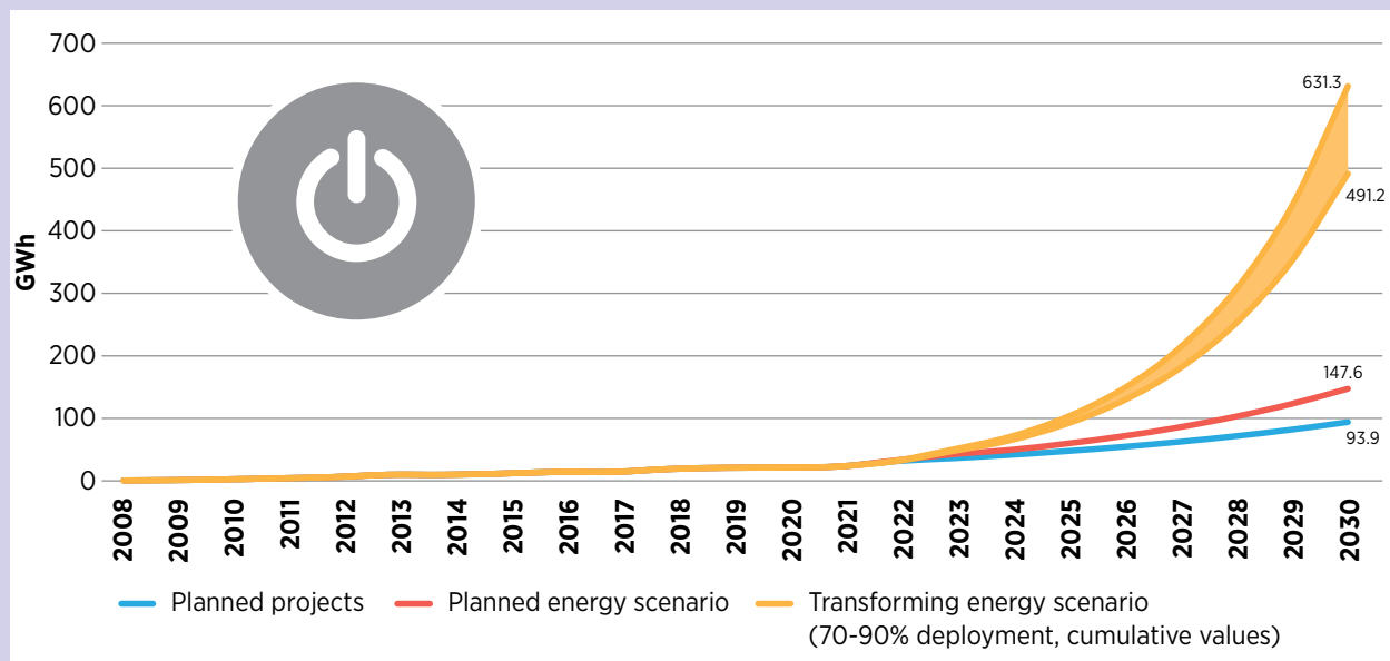
Figure 4: Molten-salt TES installed capacity
