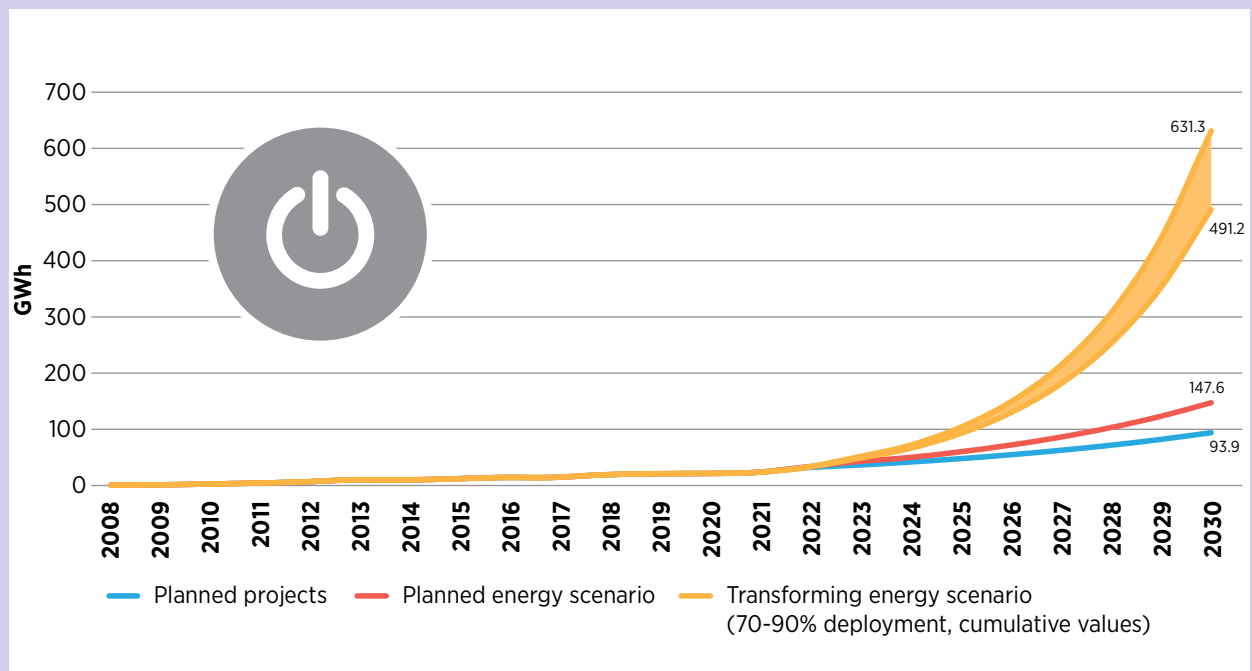
Figure 17: Installed molten-salt TES capacity
