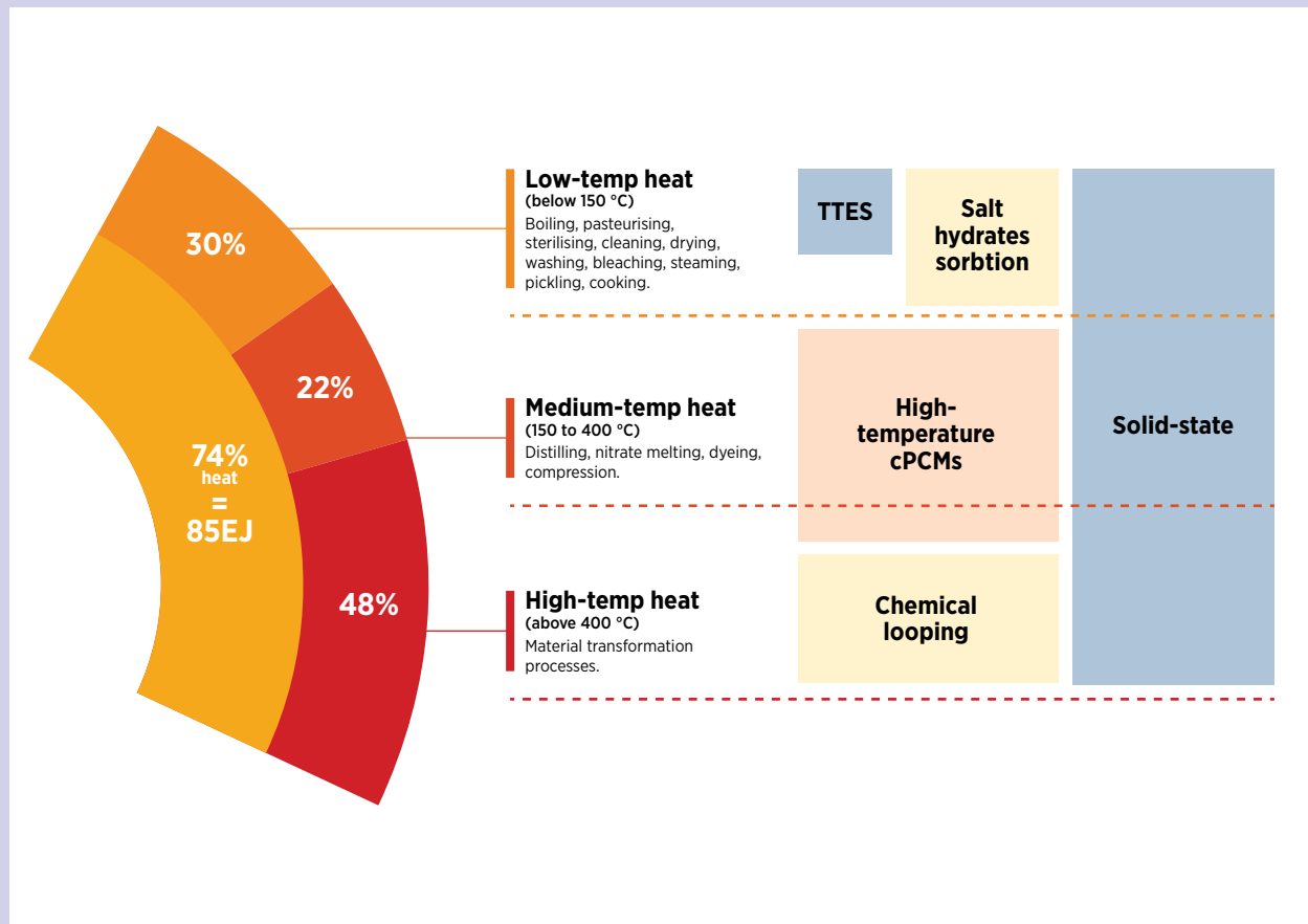
Figure 40. Technologies applicable in the industrial sector by operating temperature range
