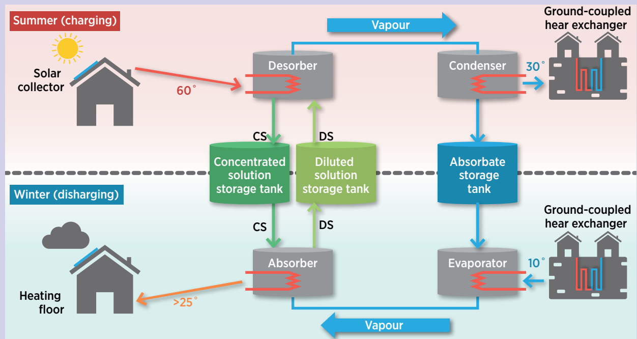
Figure 53. Absorption storage system scheme
