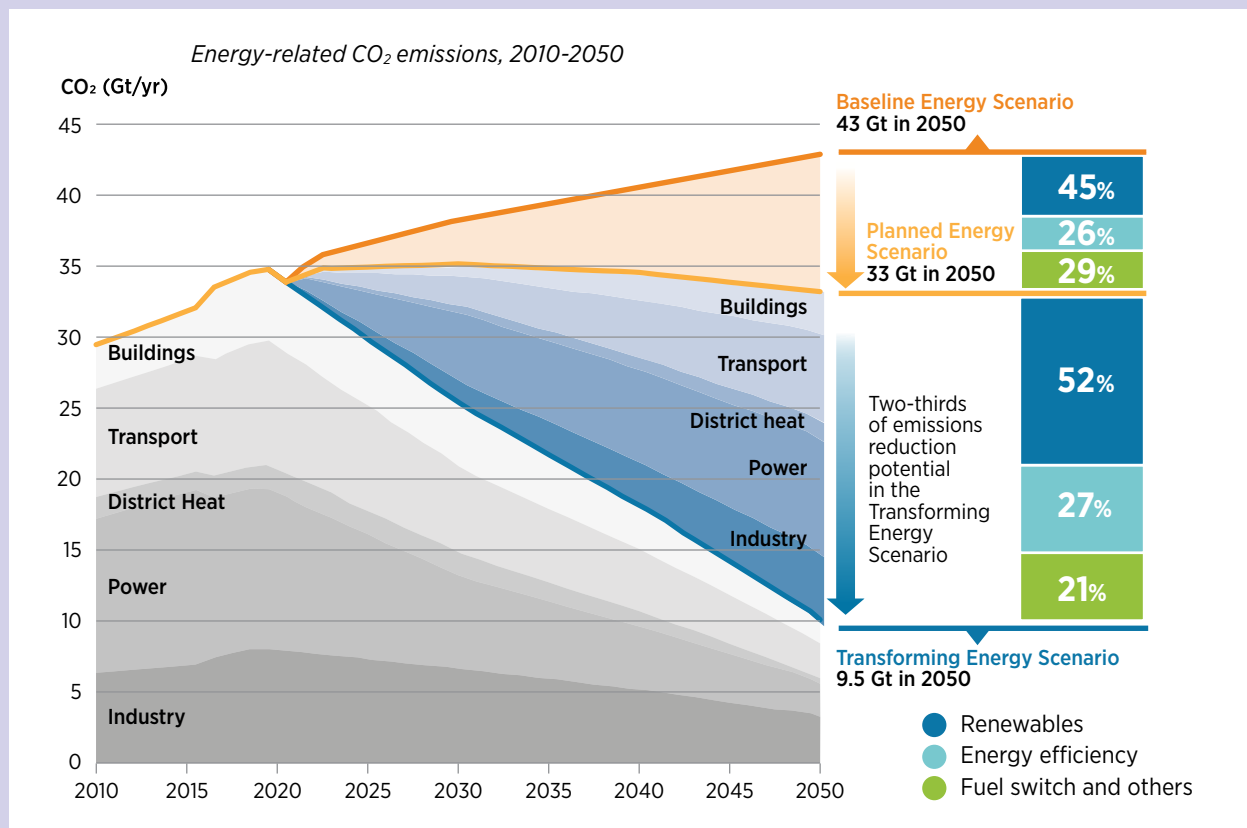
Figure 1 Appendix: Annual energy-related CO 2 emissions, 2010-2050 (Gt/yr)
