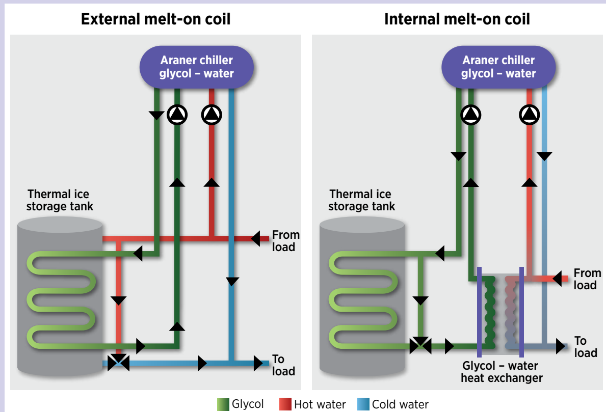
Figure 29: Ice-on-coil system
