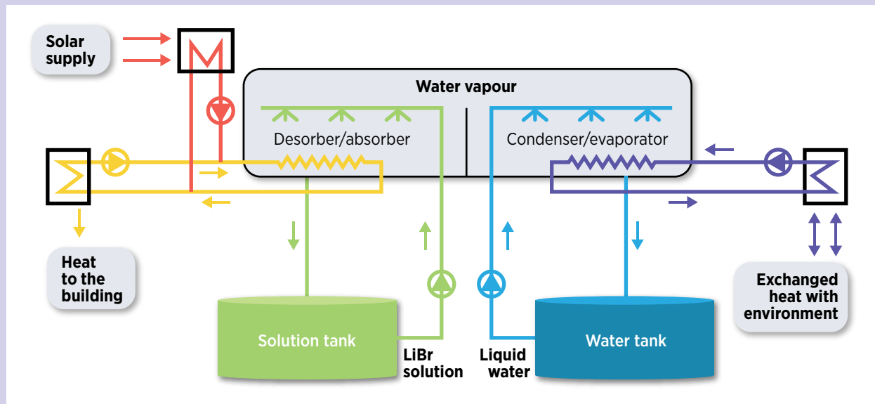
Figure 52. Process configuration with separator reactor concept
