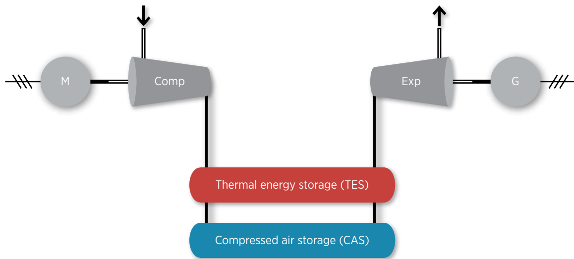
Figure 54. Adiabatic CAES with TES
