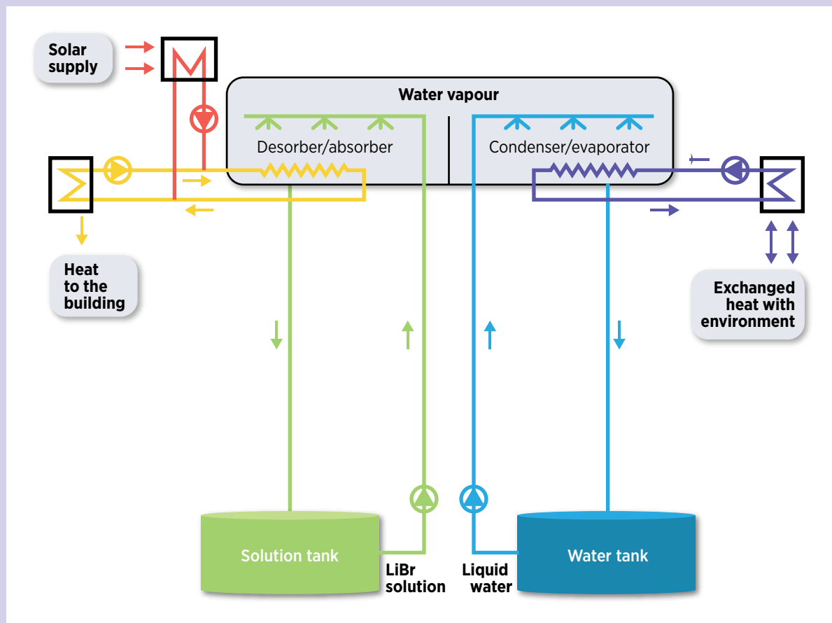
Figure 33: Absorption system configuration with separator reactor
