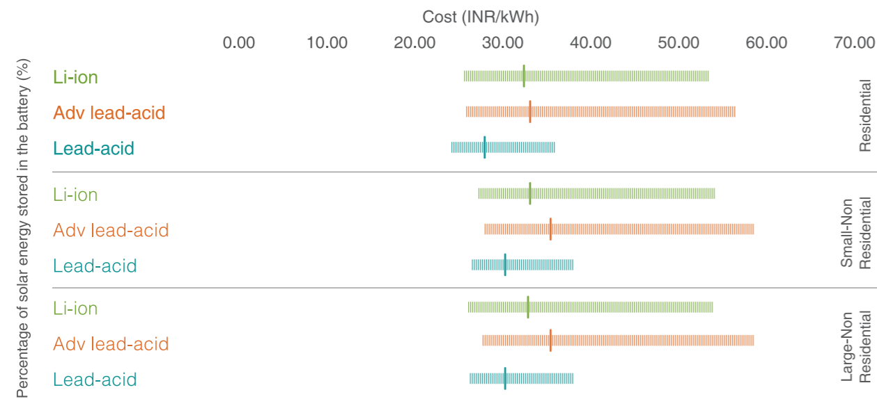
Figure 2: Cost of standalone energy storage.
