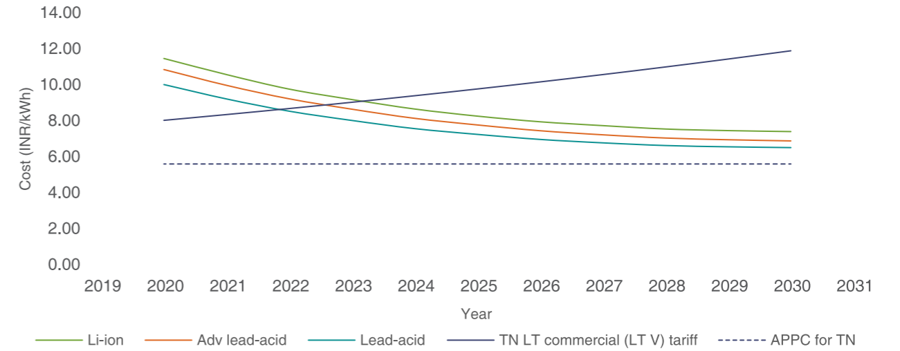
Figure ES.2: Projected decline in the levelised cost of solar plus energy storage for the Small Non-Residential user case, in the case of 30% of solar energy flowing through the battery.
