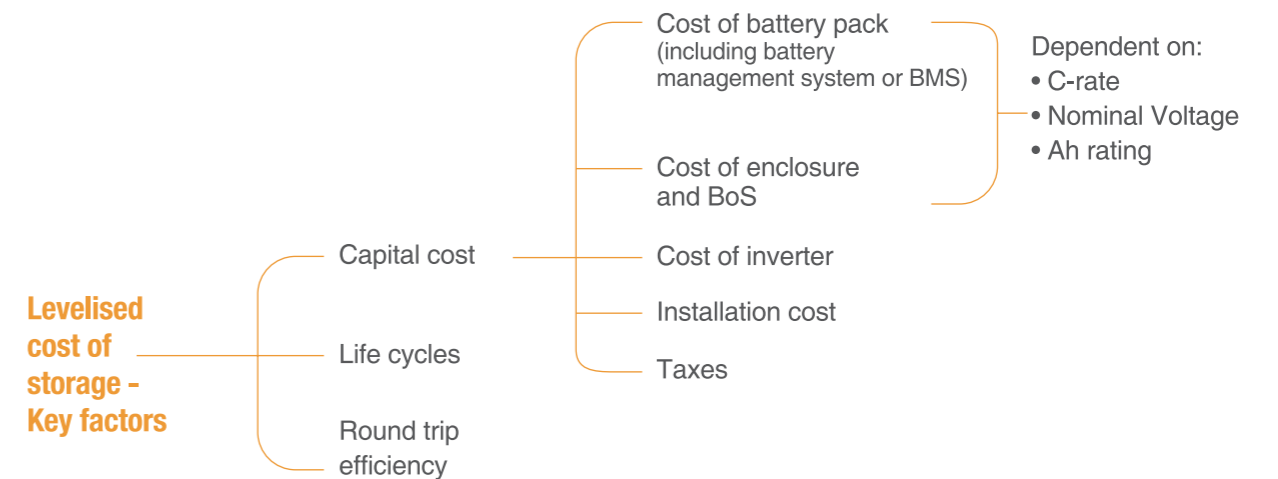
Figure 1: Key factors for levelised cost of storage of a battery energy storage system.
